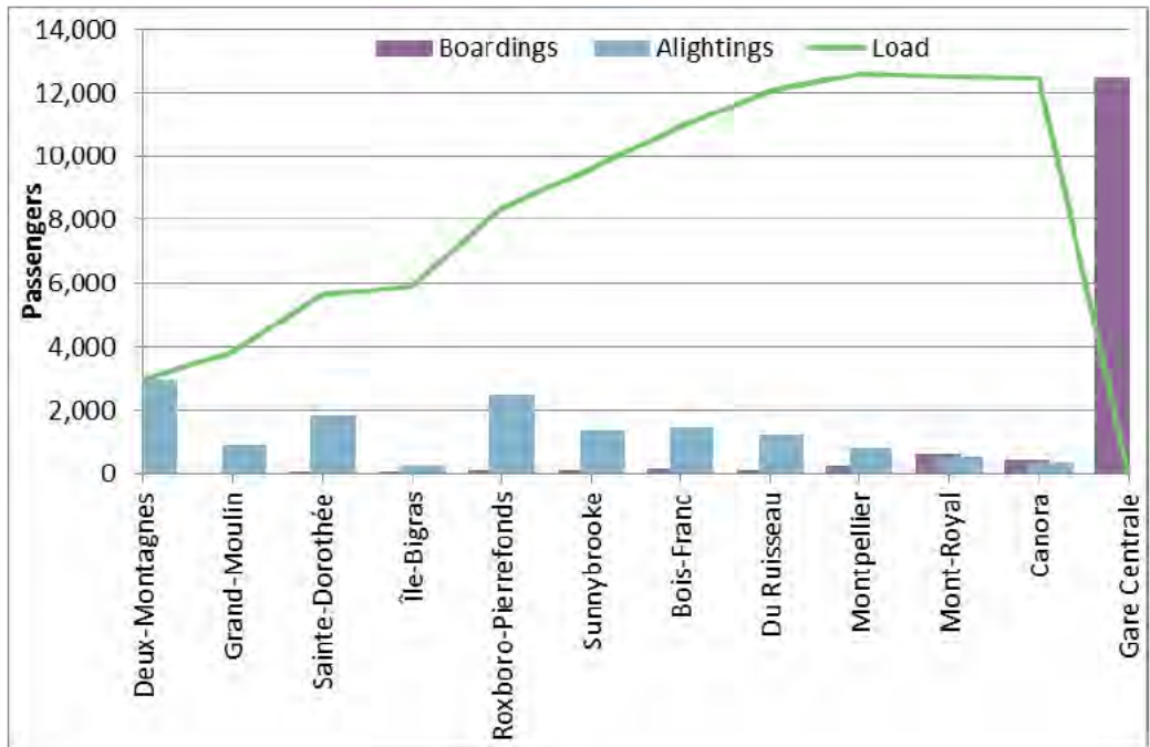
Figure 3-7: Deux-Montagnes Line AM Peak Profile (Sept 11th 2014) – Towards Downtown Montréal
